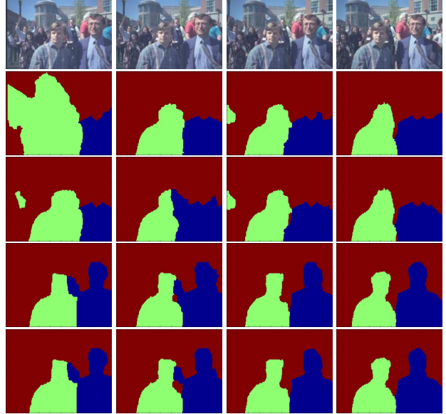
Figure 5. Segmentation results of the 'Dayton' sequence. Rows 2 and 3 show the results obtained for the frames shown in row 1 by minimizing the energy function in equation (39) using \alpha\beta -swap and \alpha -expansion respectively. Row 4 and 5 show the segmentations obtained by minimizing the energy in equation (42) using \alpha\beta -swap and \alpha -expansion respectively. The use of higher order cliques results in more accurate segmentation.
