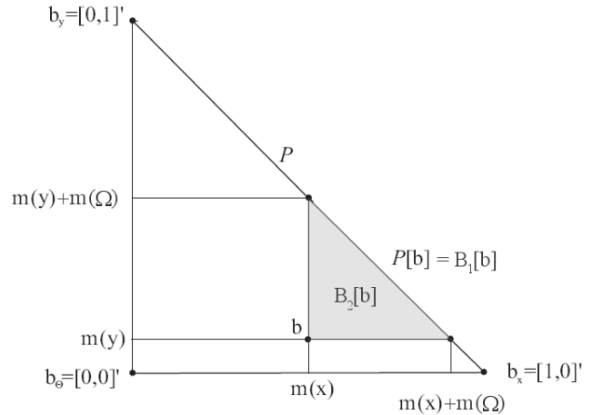
Figure 1. The polytope \mathcal{B}_2[b] of the 2-additive belief functions dominating a given belief function b defined on a frame of size 2. The vertices of such polytope meet the conjectured form (7), and are given by the basic probability assignments of Equation (8).
